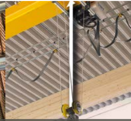
Minimum hook travel
